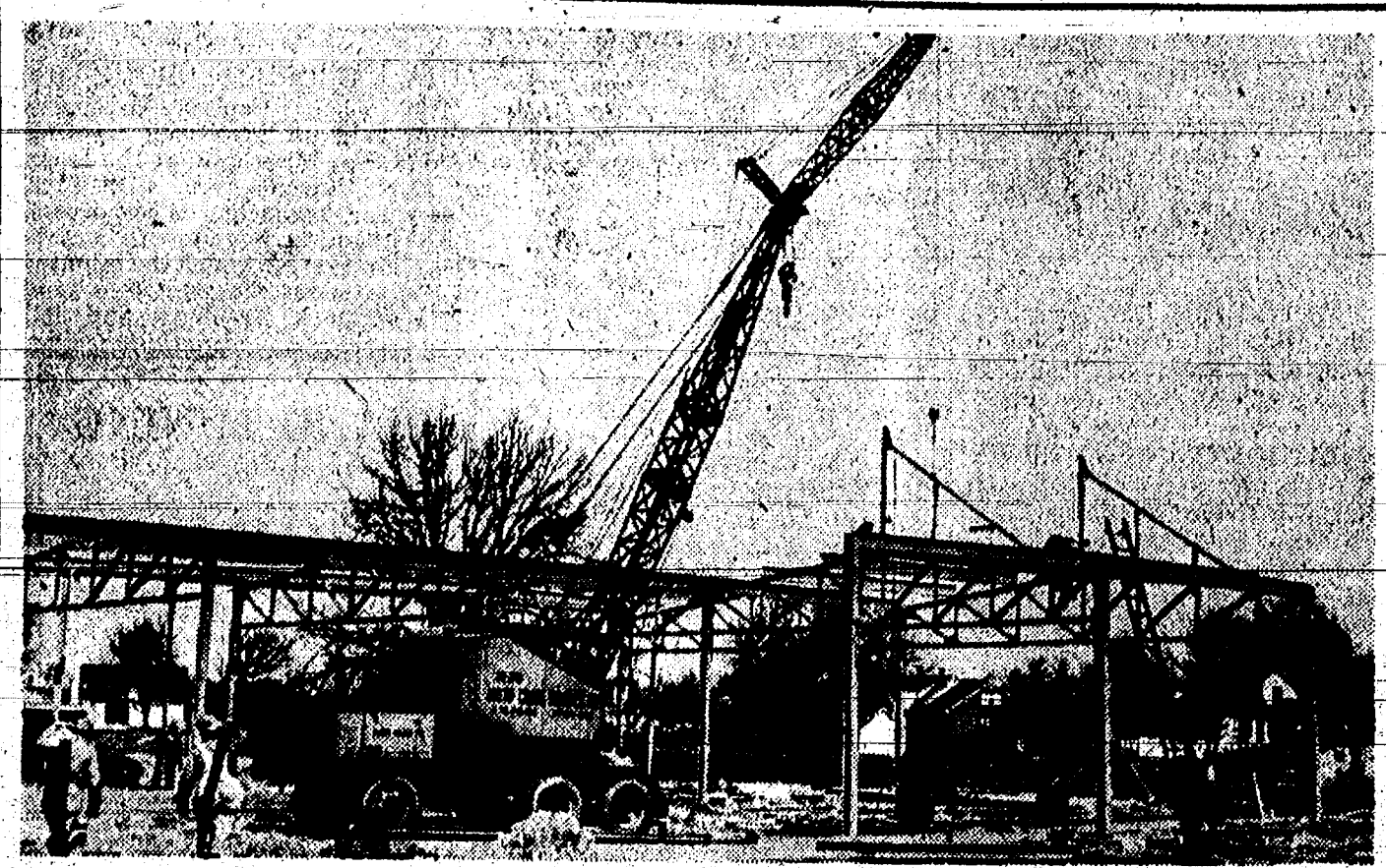
CONSTRUCTION WORK began in earnest on the new addition to the Chelsea Spring Company's plant last week when workmen began erecting the steel framework as shown above. The addition will add about 45,000 square feet of floor space and will house additional equipment made necessary in their general expansion program.
